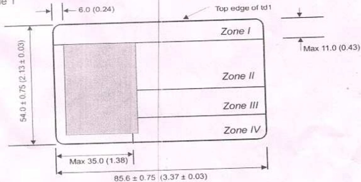
Figure 6: Specification of Zone on front page of size1 card
