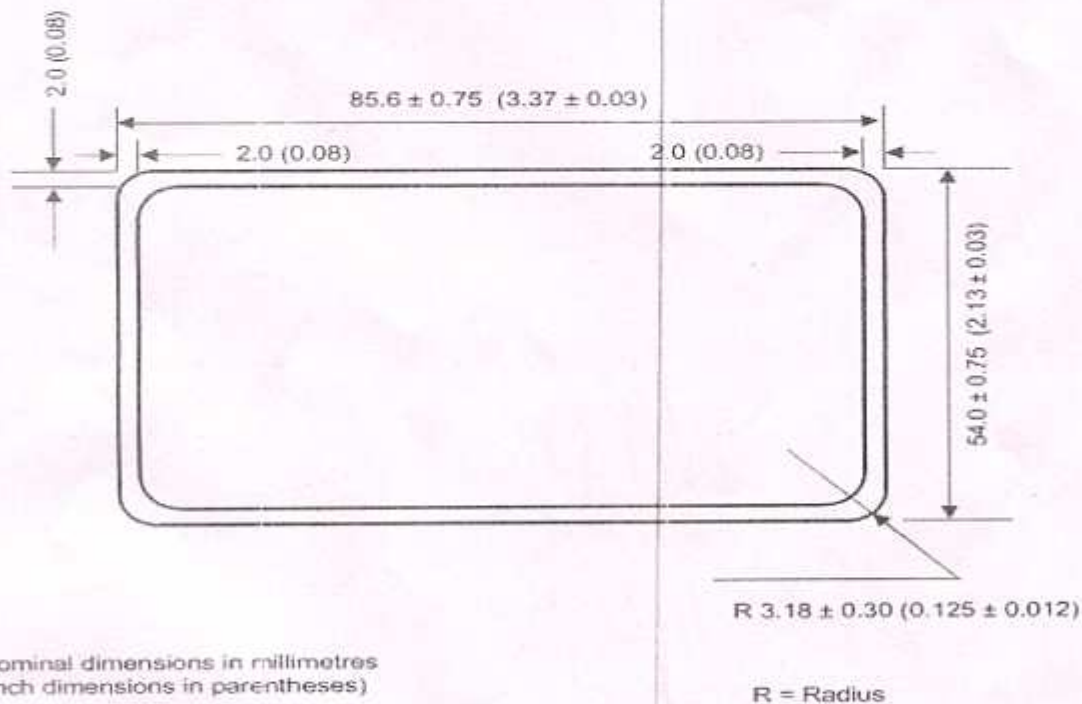
Figure 1 : Inner and Outer dimension of card of size1
